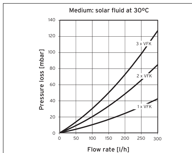
Fig. 4.8 Pressure loss auroTHERM VFK 900, VFK 990/1
