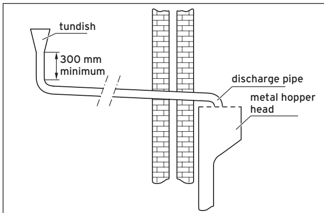
Fig. 5.18 High discharge connection
