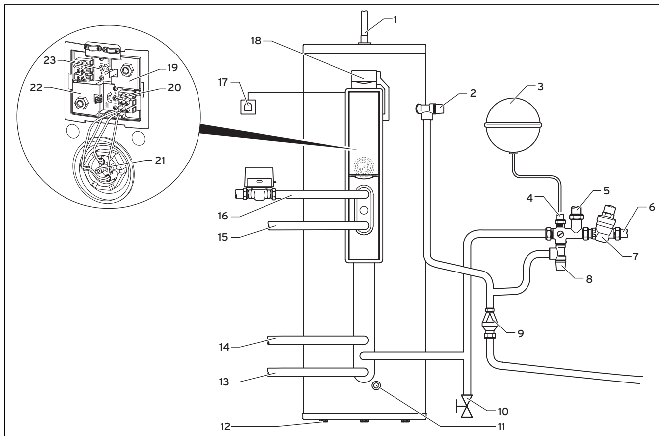
Fig. 5.1 auroSTOR function elements
