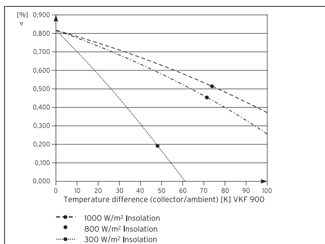
Fig. 4.7 Efficiency according to DIN EN 12975
