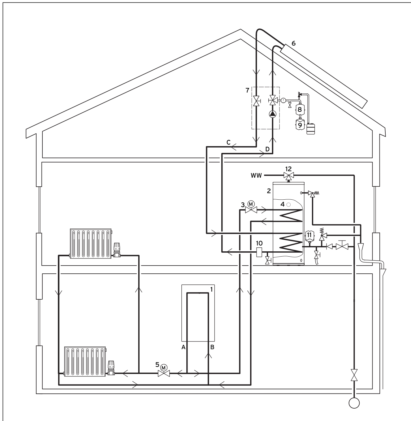
Fig. 5.9 Functional diagram
