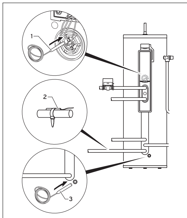
Fig. 5.23 Installation of the VR 10 temperature sensor
