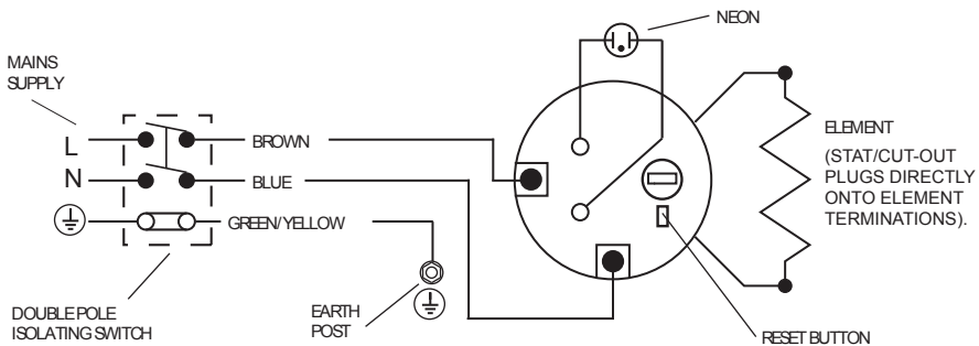
FIGURE 06: WIRING DIAGRAM
