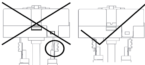
FIGURE 07: THERMOSTAT INSTALLATION
